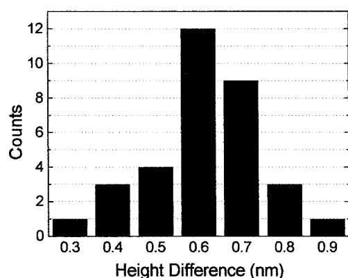
FIGURE 6 Histogram of the apparent height differences before and after the molecules were imaged in the repulsive interaction regime. In all cases, the apparent height at its maximum value has been measured from images taken in the attractive interaction regime. Each molecule has been imaged twice in the repulsive interaction regime.
