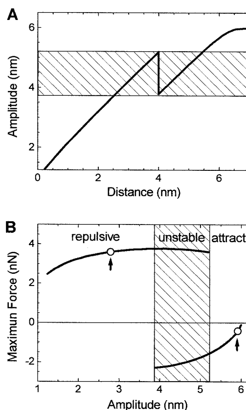
FIGURE 7 ( A ) Theoretical amplitude dependence on tip-sample separation. The shadowed region indicates the values of the oscillation amplitude that produce an unstable behavior. ( B ) Calculated maximum force dependence on the oscillation amplitude. The arrows indicate the values of the experimental setpoint amplitudes used for recording the images shown in Fig. 5.
